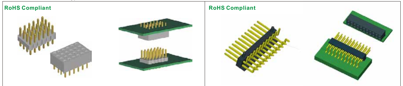
1999P-XXG No. Of Positions P: Male S: Female 1999 Series: 2.0mm 4Rows Pin Header & PCB Socket Mating Part: 1999P-XXG Mating 1999S-XXG
