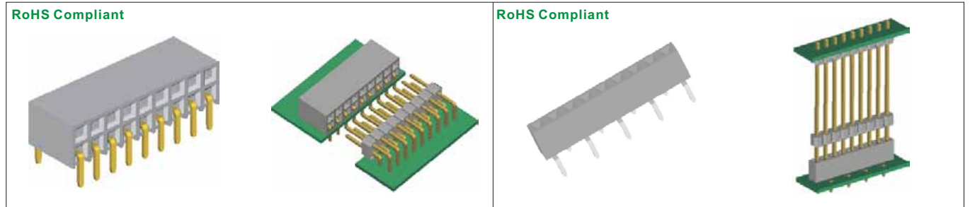
2214BR-XXG No. Of Positions Double Rows 2214BR Series: 2.54mm PCB Socket Horizontal Entry Mating Part: 2214BR-XXG Mating 2213 Series 2212TB-XXG-XX B1&B2 Type No. Of Positions Bottom Entry 2212TB Series: 2.54mm PCB Socket Bottom Entry Mating Part: 2212TB-XXG-XX Mating 2211 Series
