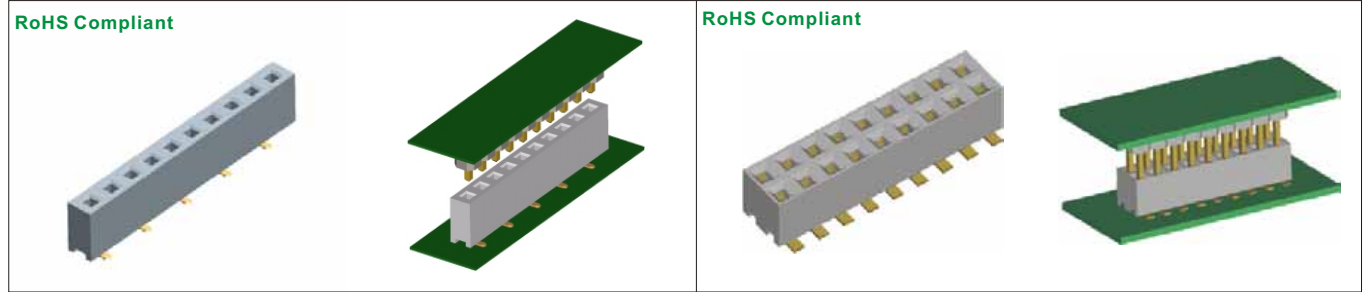
2212SM-XXG-50-BX B1 & B2 Type No. Of Positions Single Row SMD 2212SM-XXG-50-BX Series: 2.54mm PCB Socket SMD Type 5.0mm height Mating Part: 2212SM-XXG-50-BX Mating 2211 Series 2214SM-XXG-50 No. Of Positions Double Rows SMD 2214SM-XXG-50 Series: 2.54mm PCB Socket SMD Type 5.0mm height Mating Part: 2214SM-XXG-50 Mating 2213 Series
