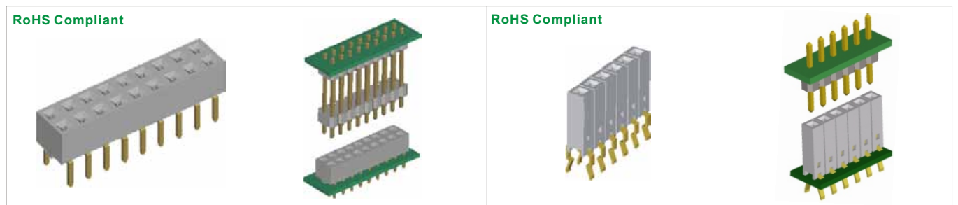
2214TB-XXG-XX Row to Row Space 03:3.81 / 05:5.08 07:7.62 No. Of Positions Bottom Entry 2214TB Series: 2.54mm PCB Socket Bottom Entry Mating Part: 2214TB-XXG-XX Mating 2213 Series 2212TBA-XXG-XX Pitch Type 02:3.17mm 04:3.96mm 05:5.08mm No. Of Positions 2212TBA Series: 2.54mm PCB Socket 3 Side Contact 8.5mm height Mating Part: 2212TBA-XXG-XX Mating 2211 Series
