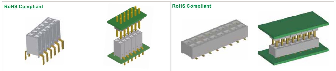
2214TBA-XXG-XX Row to Row Space 06:6.50mm 07:7.62mm No. Of Positions 2214TBA Series: 2.54mm PCB Socket 3 Side Contact 8.5mm height Mating Part: 2214TBA-XXG-XX Mating 2213 Series 2214SM-XXG-37D No. Of positions Double Rows SMD 2214SM-XXG-37D Series: 2.54mm PCB Socket SMD Type 3.7mm height Mating Part: 2214SM-XXG-37D Mating 2213 Series
