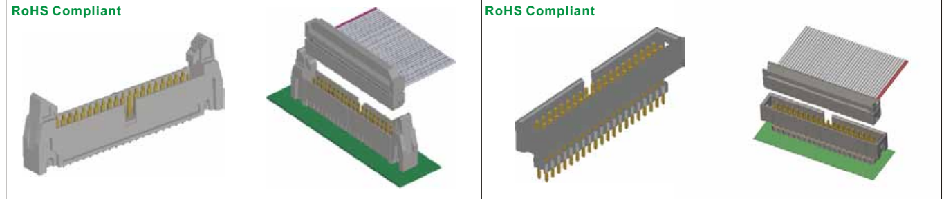
2216S-XXG-XX 00:W/O Ejector 01:Short Ejector 02:Long Ejector No. Of Positions S: Straight Type R: R/A Type 2216S Series: 2.54mm Shrouded Header With Eject Lever Mating Part: 2216S-XXG-XX Mating 4401 Series
