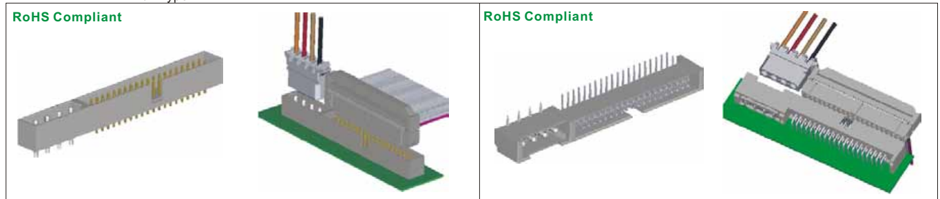
2392-2100 2 in 1 2392-2100 Series: 2 in 1 Straight Type Mating Part: 2392-2100 Mating 4401 & 8980 Series
