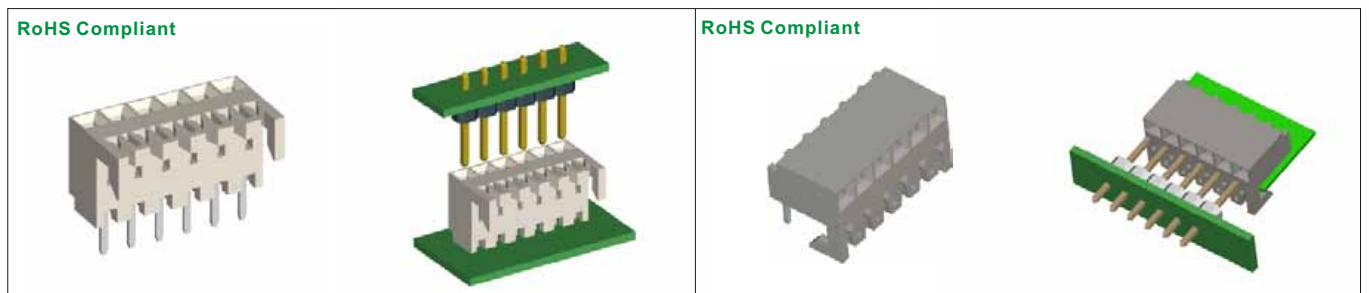
2224S-XX No. Of Positions S: Straight Type
