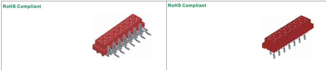
4409AR-XX No. Of Positions 4,6,8,10,12,14,16,18,20 Ways
