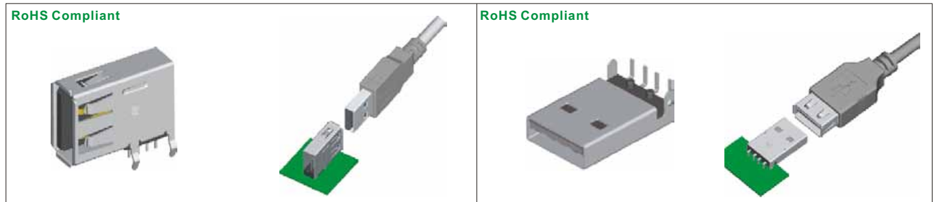
5075AUR-04-XX WH:White(Standard) BK:Black Up R/A Type 5075AUR-04-XX USB Connector A Female 4 Ways Up R/A Type Application: 5075AUR-04 Mating USB A cable
