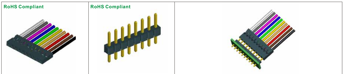
2026A-XX No. Of Positions A: Single Row B: Double Rows 2210S-XXG G: Gold Plated No. Of Positions S: Straight Type 2210: Single Row 2208: Double Rows 2026 Series: 2.0mm Mini Latch Housing Single & Double Rows 2210 & 2208 Series: 2.0mm Pin Header Single & Double Rows Mating Part: 2026A-XX Mating 2210S(R)-XX
