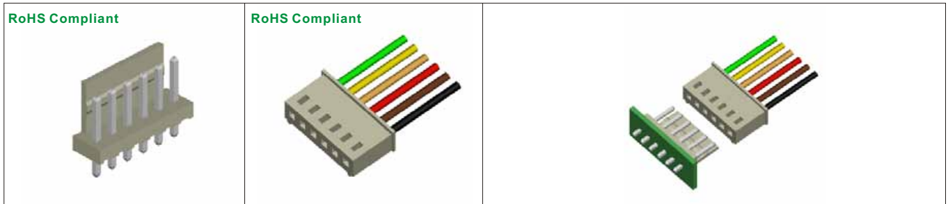
2317SB-XX No. Of Positions SB: Straight Type RB: R/A Type 2318HB-XX No. Of Positions HB: Housing 2317 Series: 2.5mm Wafer Straight & R/A Type 2318HB Series 2.5mm Housing Connector Mating Part: 2317SB-XX Mating 2318HB-XX
