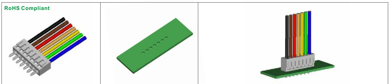
1310H-XX No. Of Positions H: Straight Type HR: R/A Type PC Board 1310 Series: 2.0mm Board-In Type Connector Mating Part: 1310H-XX Mating PCB
