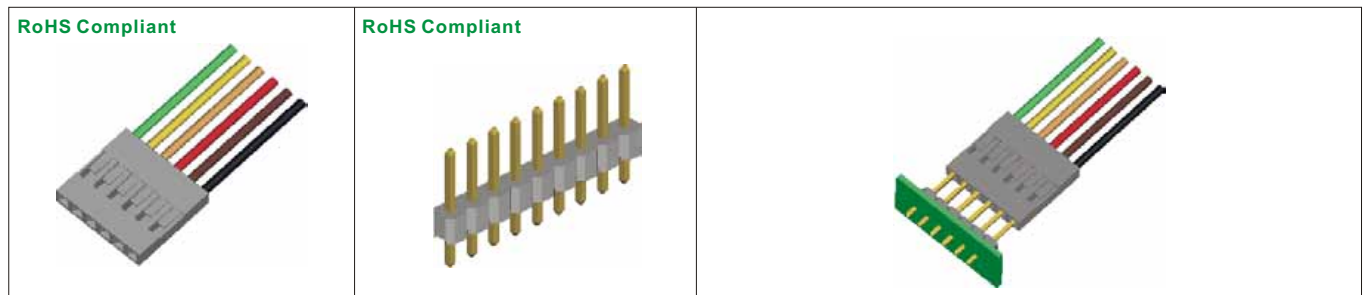
2226A-XX No. Of Positions A: Single Row B: Double Rows 2211S-XXG G: Gold Plated No. Of Positions S: Straight Type 2211: Single Row 2213: Double Rows 2226 Series: 2.54mm Housing Single & Double Rows 2211 & 2213 Series: 2.54mm Pin Header Single & Double Rows Mating Part: 2226A-XX Mating 2211S(R)-XX
