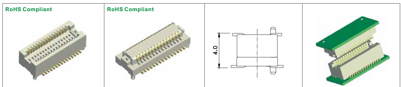
2000P-XXG-270-01 No. Of Positions Male type
